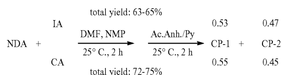
Figure 1. One-pot condensation of NDA with IA and CA in polar solvents.
